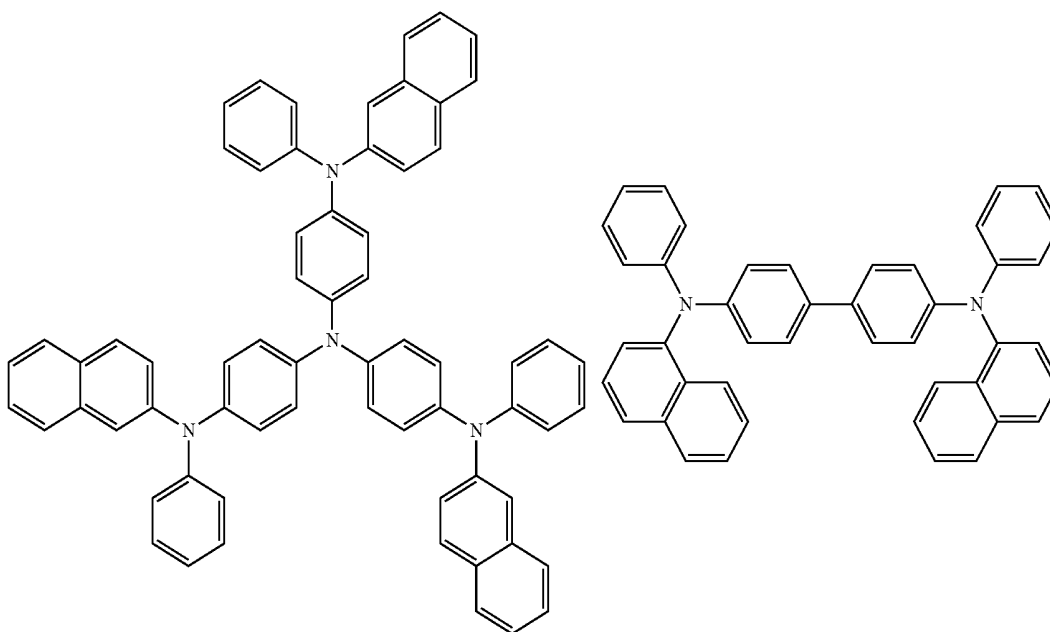
2-TNATA
